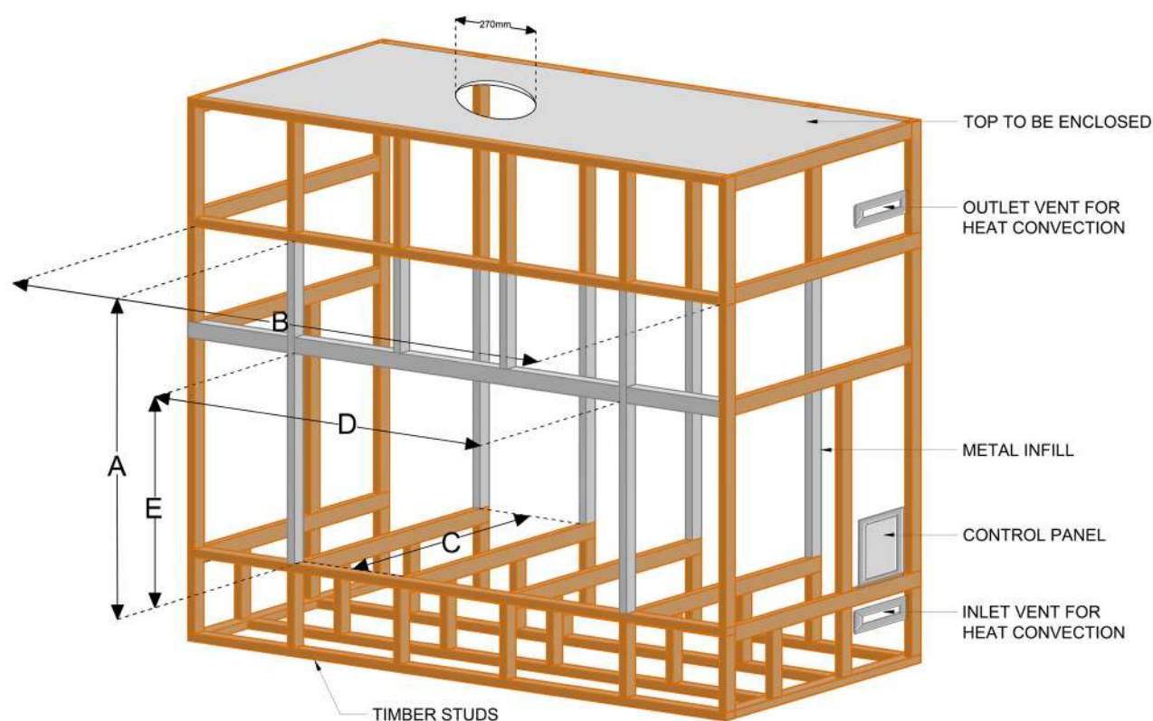
Figure 1.8 (Timber framing)
