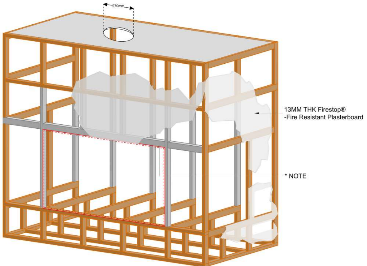
Figure 1.7 (Cladding Material)
